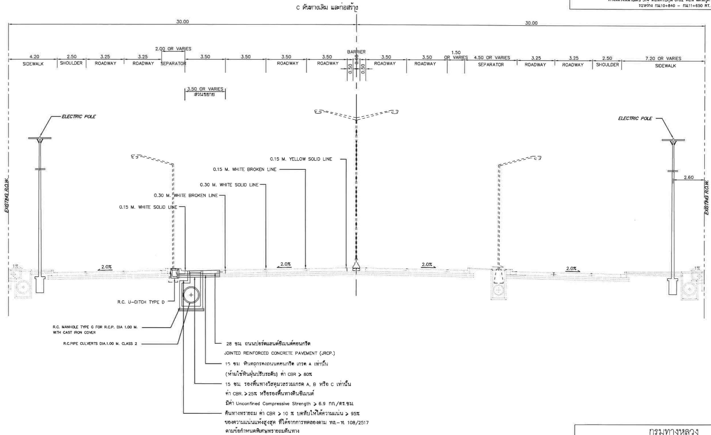
TYPICAL CROSS SECTION HW.365 AI SIA. U+3/5 (SEE DETAIL IN PLAN)
