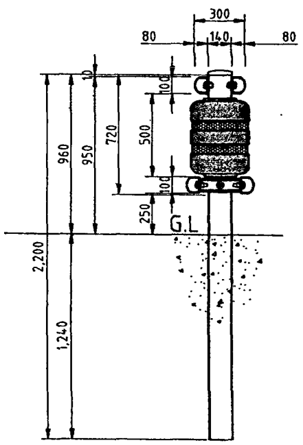
Roller System Section Not To Scale
