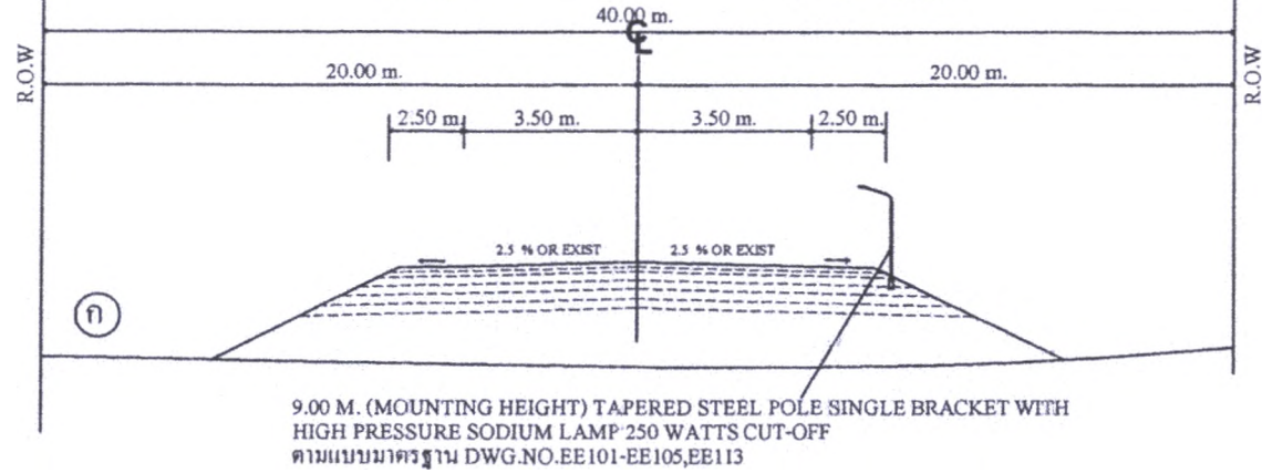
TYPICAL CROSS - SECTION A - A SCALE : NO SCALE
