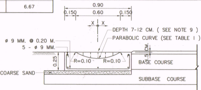
R.C. GUTTER DETAILS SCALE 1:25
