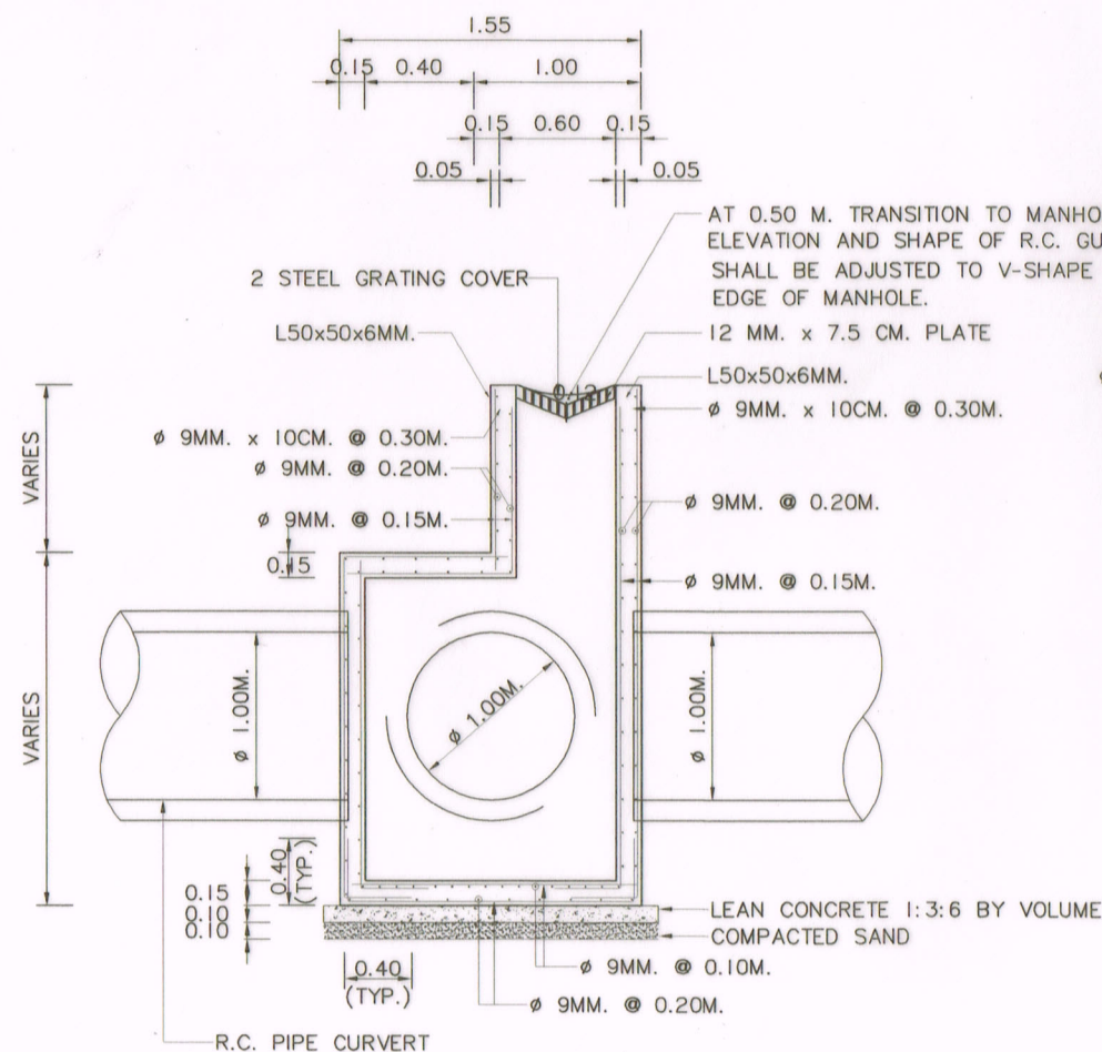
SECTION (A) - (A) SCALE 1:50
