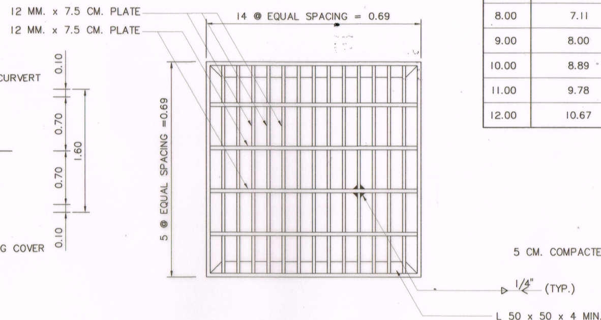
STEEL GRATING COVER DETAILS SCALE 1:25
