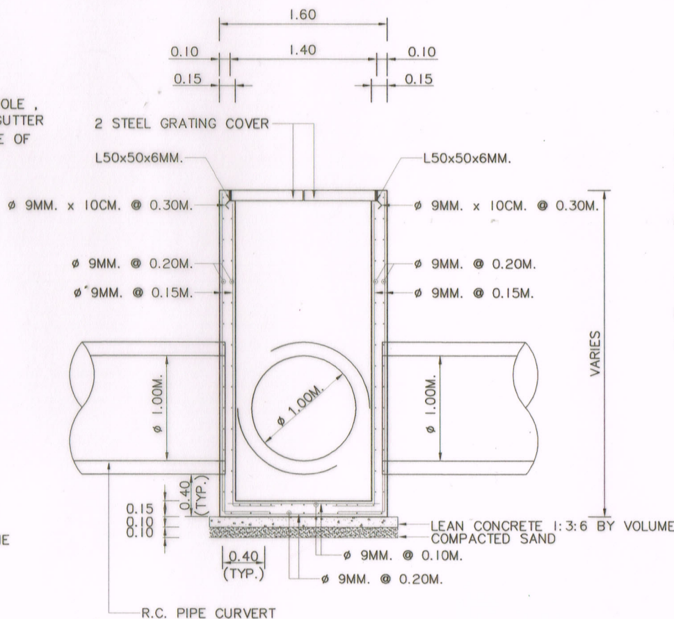
SECTION (B) - (B) SCALE 1:50
