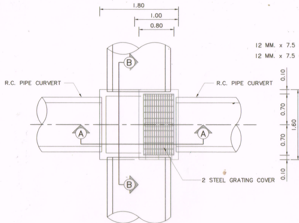
PLAN OF MODIFICATION OF R.C. MANHOLE TYPE "C" SCALE 1:50
