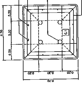
PLAN-REINFORCEMENT SCALE 1:10
