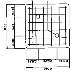
PLAN-COVER-REINFORCEMENT SCALE 1:10
