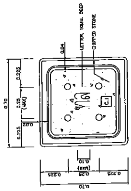
PLAN WITH COVER-HANDHOLE TYPE C.1 SCALE 1:10
