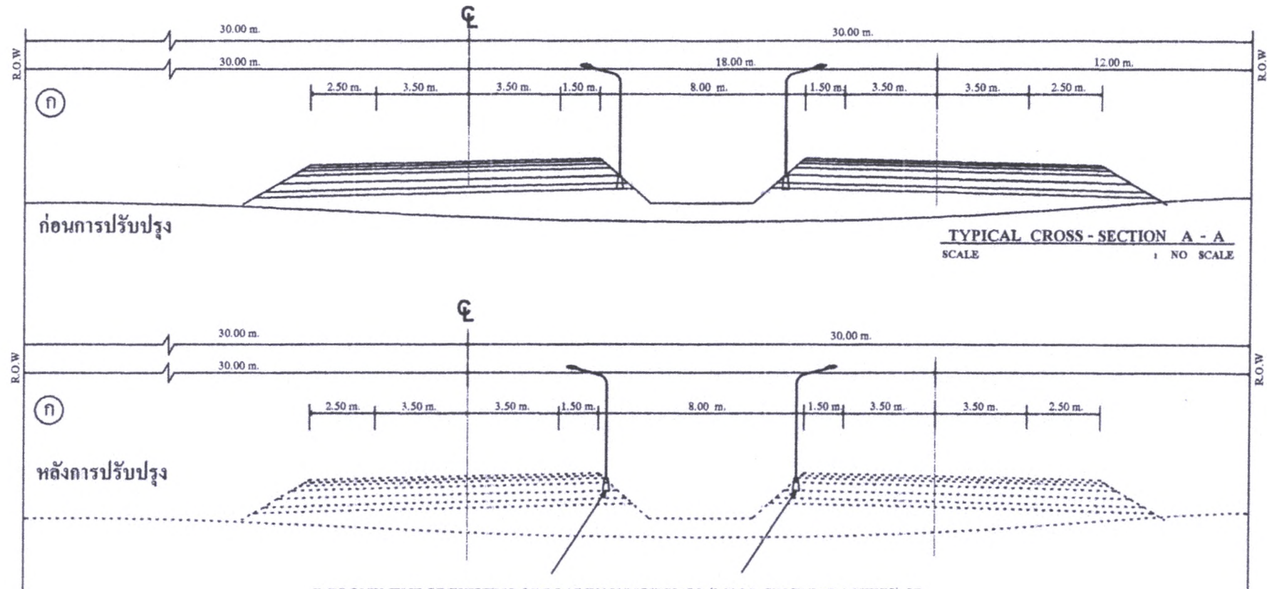
TYPICAL CROSS - SECTION A - A SCALE : NO SCALE
