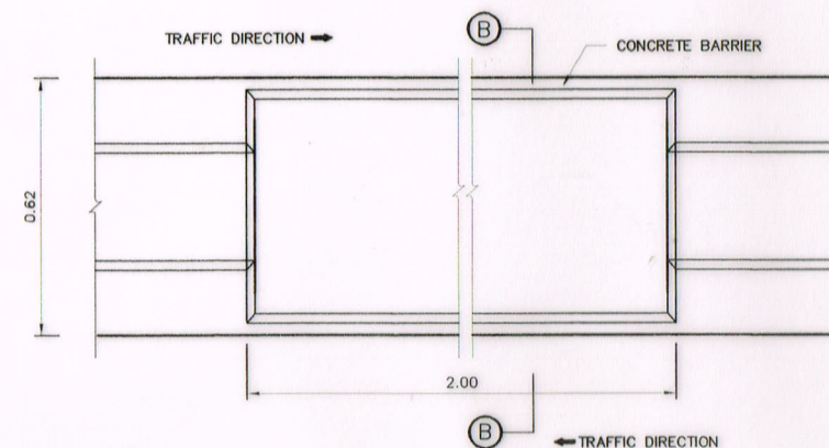
PLAN OF CONCRETE BARRIER OPEN FOR PEDESTRIAN CROSS WALK SCALE 1 : 10
