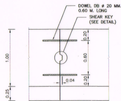
CONSTRUCTION JOINT DETAIL SCALE 1 : 20
