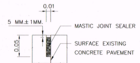
DETAIL "B" (LONGITUDINAL JOINT) NOT TO SCALE
