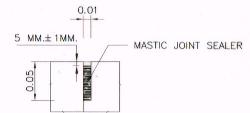
DETAIL "C" (DUMMY JOINT) NOT TO SCALE
