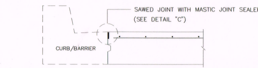
DETAIL OF DUMMY JOINT SCALE 1:20
