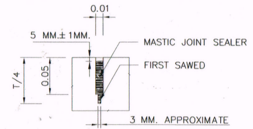
DETAIL "A" (CONTRACTION JOINT) NOT TO SCALE
