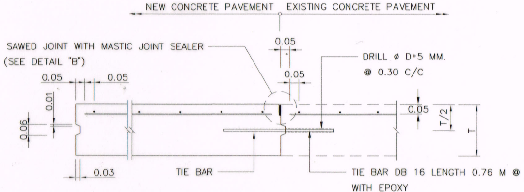
DETAIL OF MODIFICATION LONGITUDINAL JOINT SCALE 1:20
