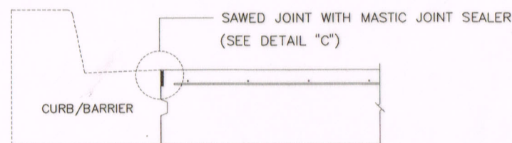
DETAIL OF DUMMY JOINT SCALE 1:20
