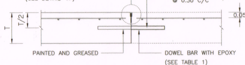
DETAIL OF MODIFICATION CONTRACTION JOINT SCALE 1:20
