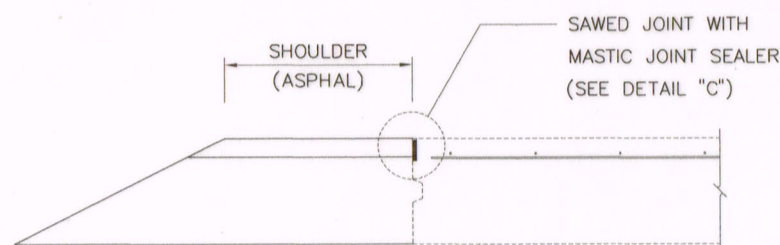
DETAIL OF EDGE JOINT SCALE 1:20
