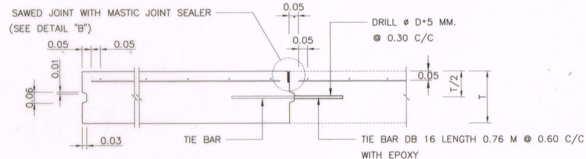
DETAIL OF MODIFICATION LONGITUDINAL JOINT SCALE 1:20
