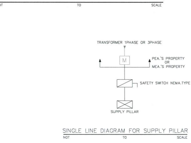
TYPICAL DIAGRAM FOR SUPPLY PILLAR 1 PHASE 2 WIRES
