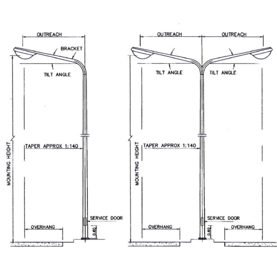
LIGHTING POLE, SINGLE ARM LIGHTING POLE, DOUBLE ARM NOT TO SCALE
