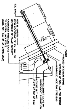
TEST NAIL/BOLT ASSEMBLY NOT TO SCALE
