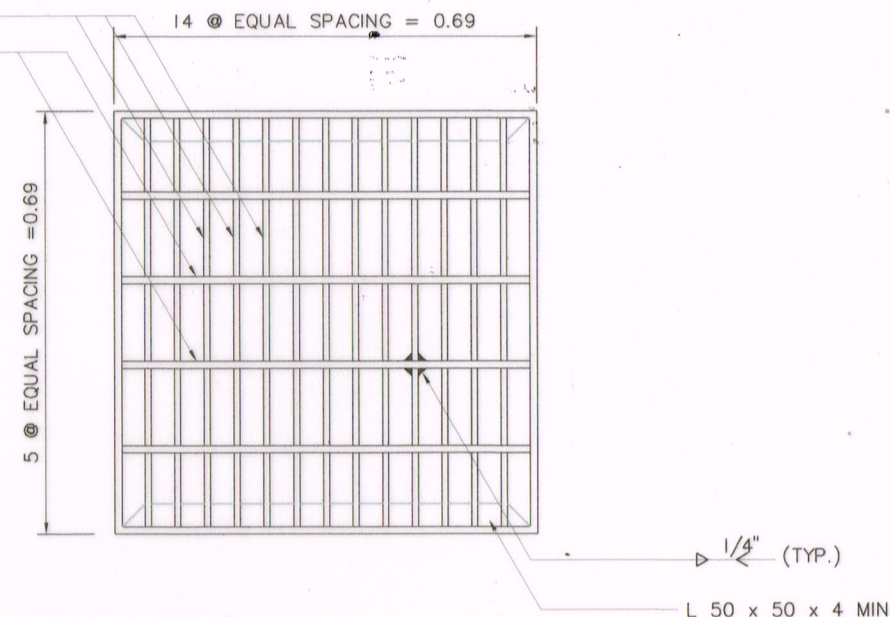
STEEL GRATING COVER DETAILS
