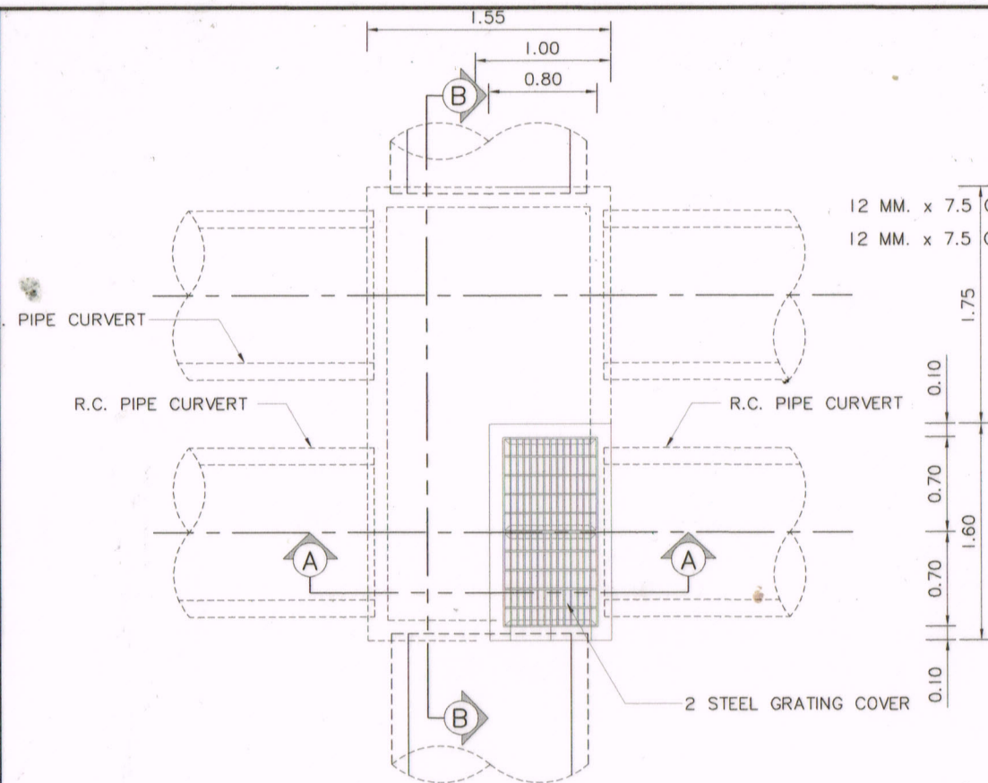
PLAN OF MODIFICATION OF R.C. MANHOLE TYPE "CA"
