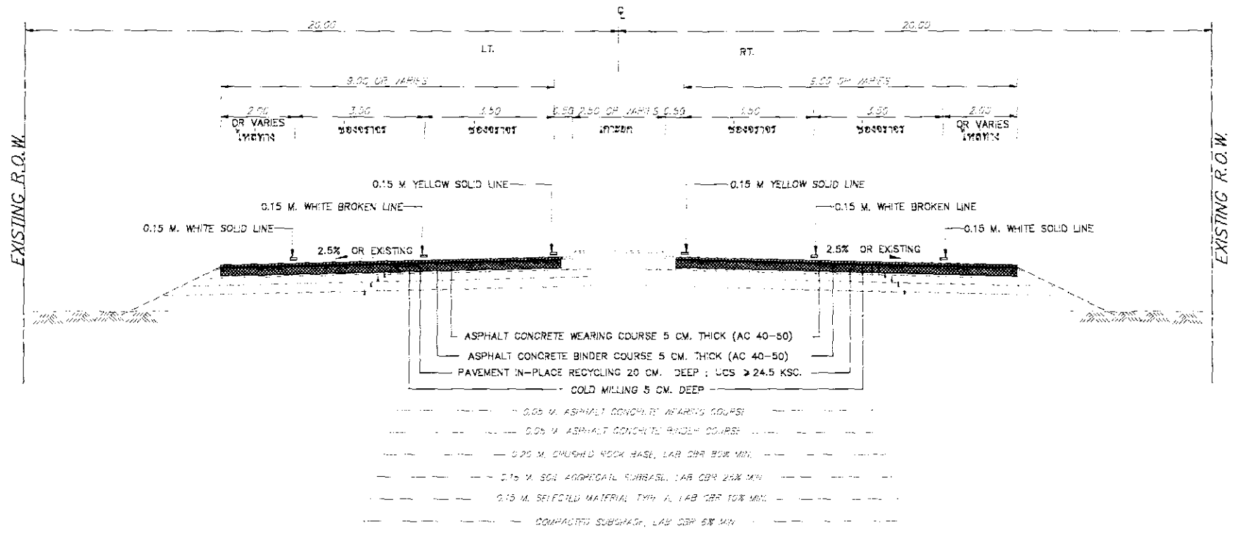
TYPICAL CROSS SECTION STA. 54+480 - STA. 54+770 NOT TO SCALE
