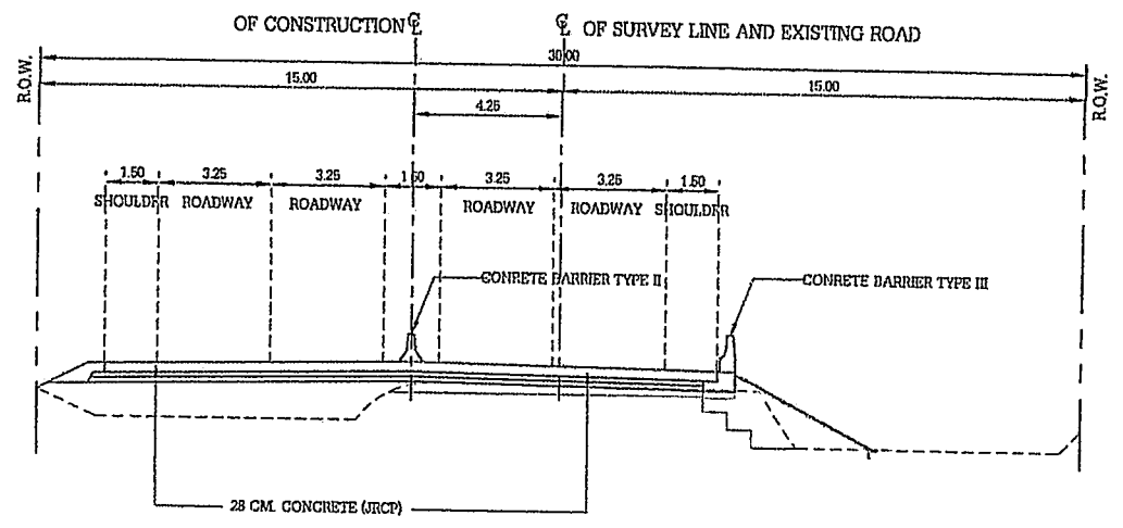
EXISTING CROSS SECTION STA.8+000 - STA.12+700
