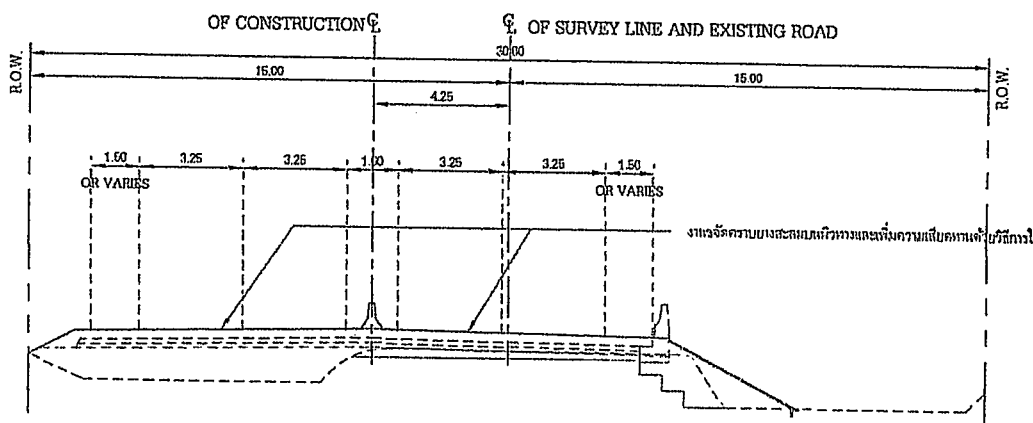
TYPICAL CROSS SECTION STA.8+000 - STA.12+700
