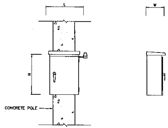
ELEVATION SUPPLY PILLAR ON CONCRETE POLE NOT TO SCALE
