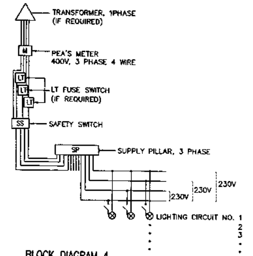
BLOCK DIAGRAM 4
