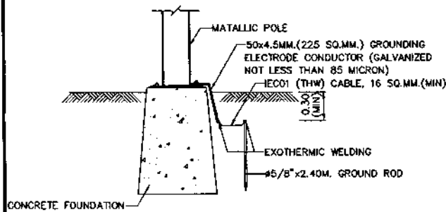
GROUNDING DETAILS
