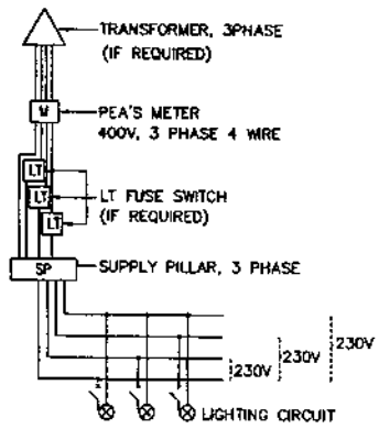
BLOCK DIAGRAM 2
