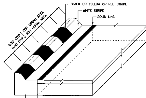
(SEE NOTE 7.) CURB MARKING DETAIL NOT TO SCALE
