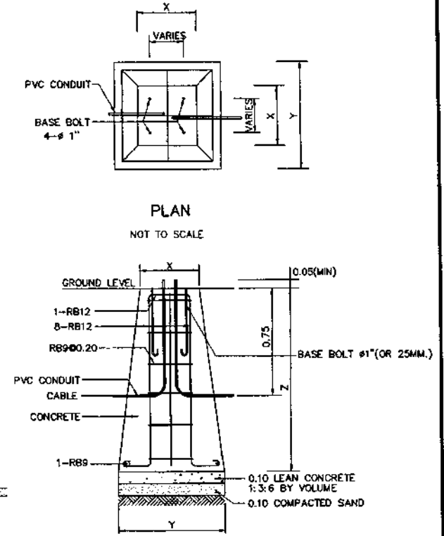
LIGHTING POLE FOUNDATION DETAILS
