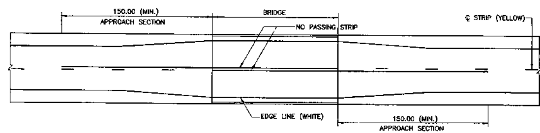
MARKING AT BRIDGE APPROACH NOT TO SCALE
