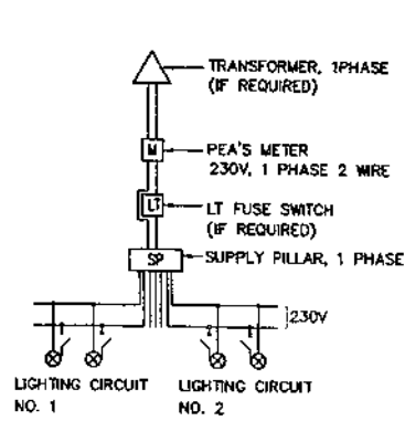
BLOCK DIAGRAM 1
