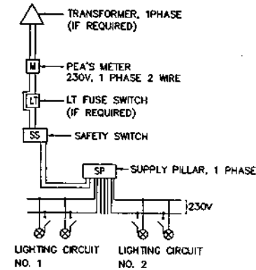
BLOCK DIAGRAM 3
