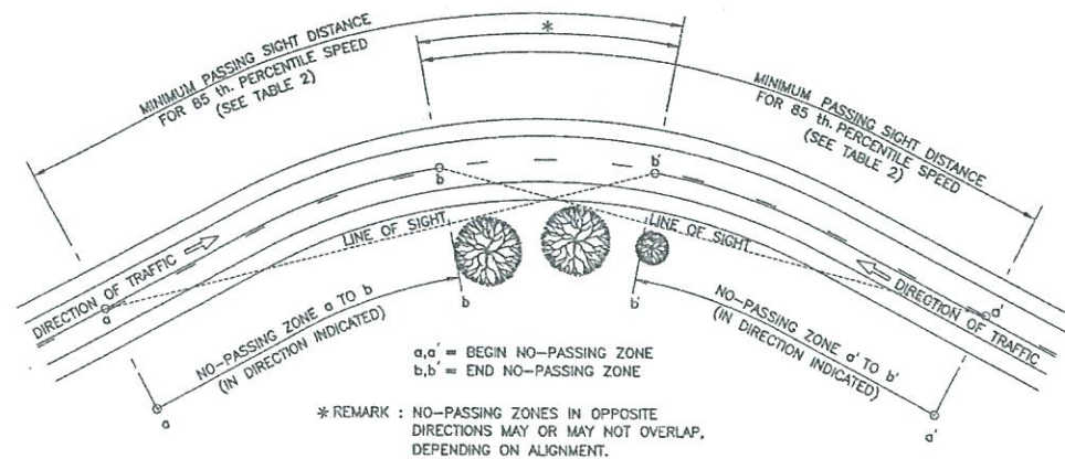
CENTER LINE MARKING FOR NO-PASSING ZONES AT HORIZONTAL CURVES
