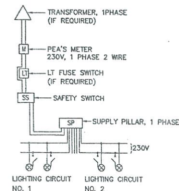
BLOCK DIAGRAM 3
