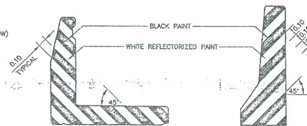
MARKING AT ENDS OF BRIDGE BARRIER
