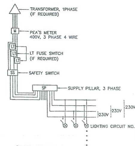
BLOCK DIAGRAM 4
