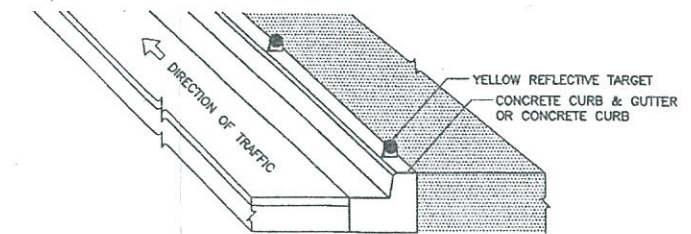
INSTALLATION REFLECTIVE TARGET ON CURB MEDIAN
