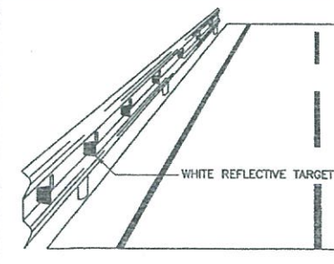
INSTALLATION REFLECTIVE TARGET ON GUARDRAIL
