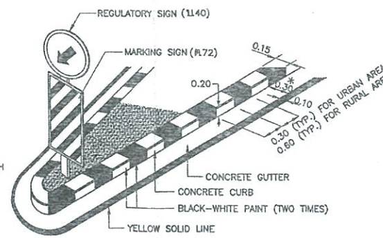
MARKING AT ENDS OF BRIDGE BARRIER
