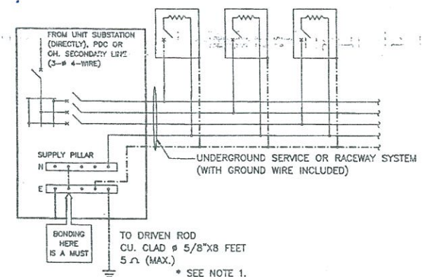
METHOD D : LIGHTING FOR ELEVATED ROAD (LIGHTING POLE/COLUMN INACCESSIBLE TO PUBLIC) & ROAD TUNNEL (LIGHTING LUMINAIRE)
