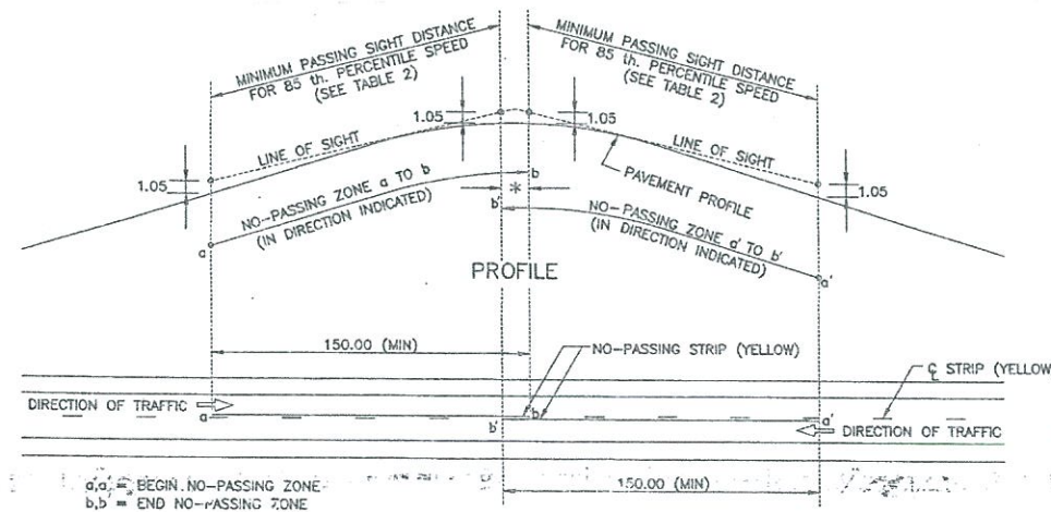
CENTER LINE MARKING FOR NO-PASSING ZONES AT VERTICAL CURVES
