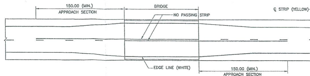
MARKING AT BRIDGE APPROACH
