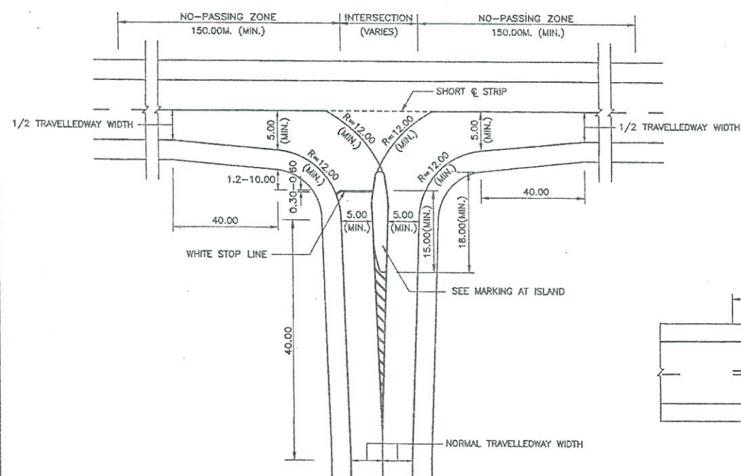
TYPICAL MARKING AT JUNCTION WITH DIVISIONAL ISLAND
