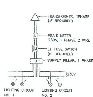
BLOCK DIAGRAM 1
