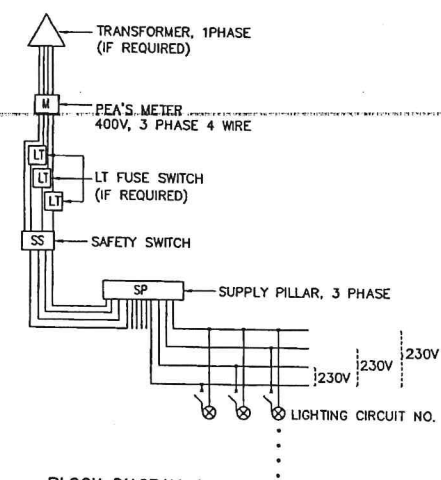
BLOCK DIAGRAM 4
