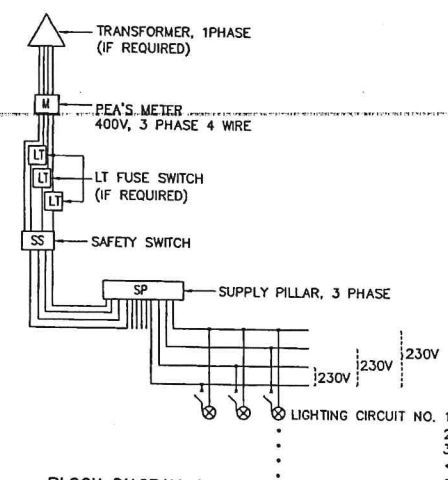
BLOCK DIAGRAM 4
