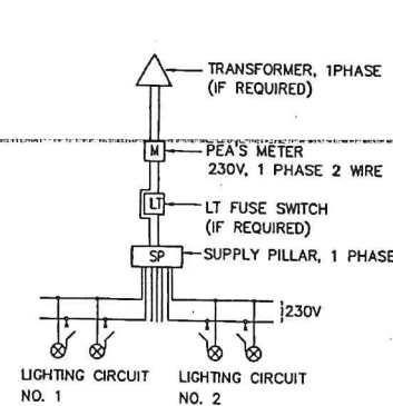
BLOCK DIAGRAM 1
