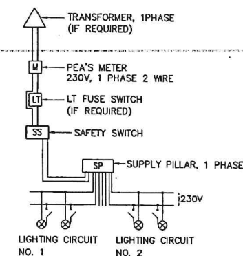
BLOCK DIAGRAM 3
