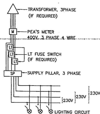
BLOCK DIAGRAM 2
