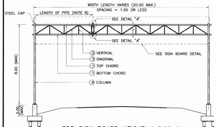
FOR SIGN BOARD HEIGHT \leq 3.00 M.
