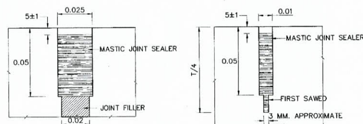
DETAIL "A" (EXPANSION JOINT)
