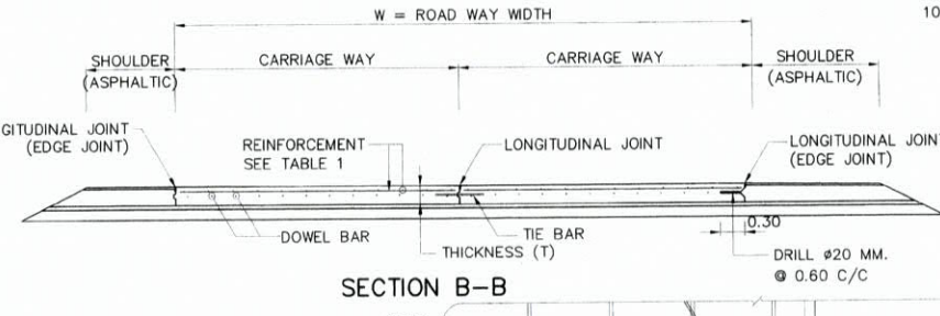
PLAN AND SECTION JOINT REINFORCED CONCRETE PAVEMENT (JRCP)
