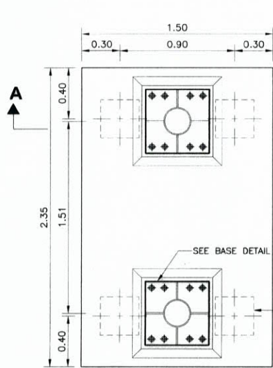
PILE FOOTING PLAN SCALE 1:20
