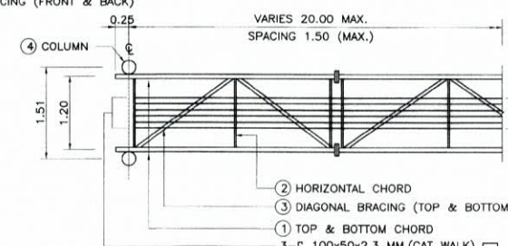
TRUSS PLAN SCALE 1:50
