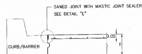
DETAIL OF DUMMY JOINT
