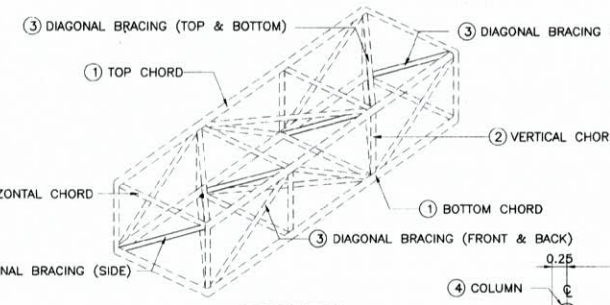
ISOMETRIC SCALE 1:50
