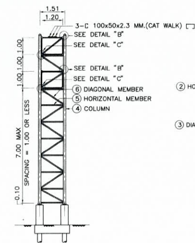
SIDE ELEVATION SCALE 1:100
