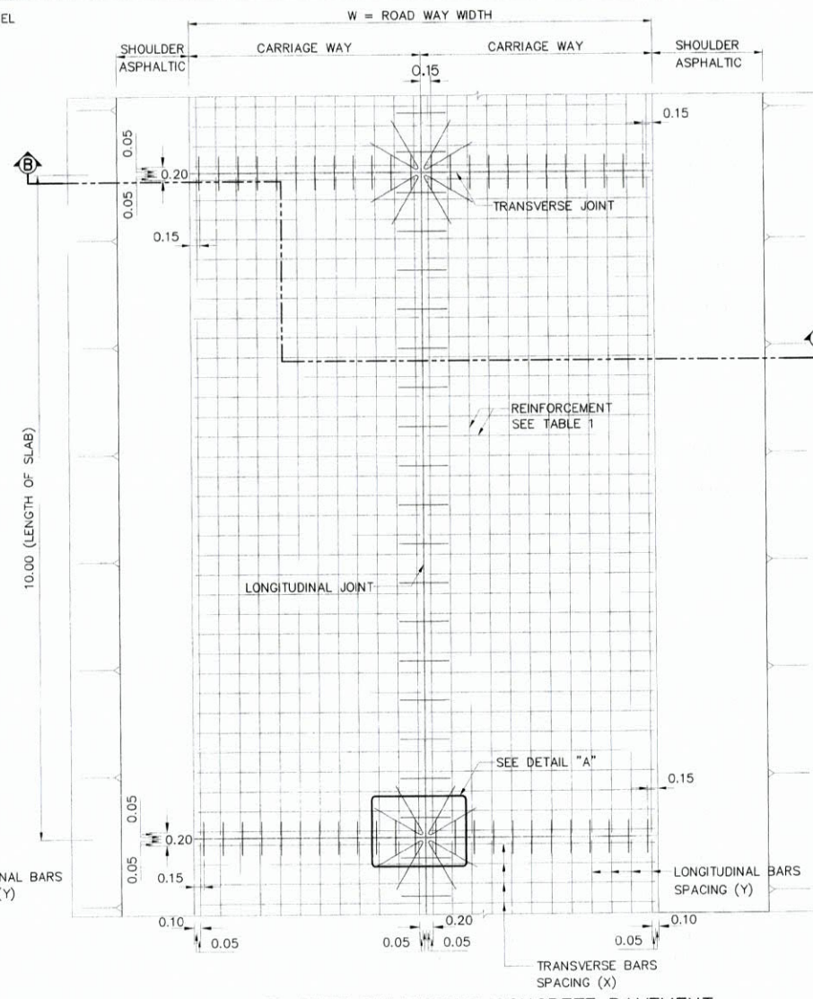
PLAN OF JOINT REINFORCED CONCRETE PAVEMENT
