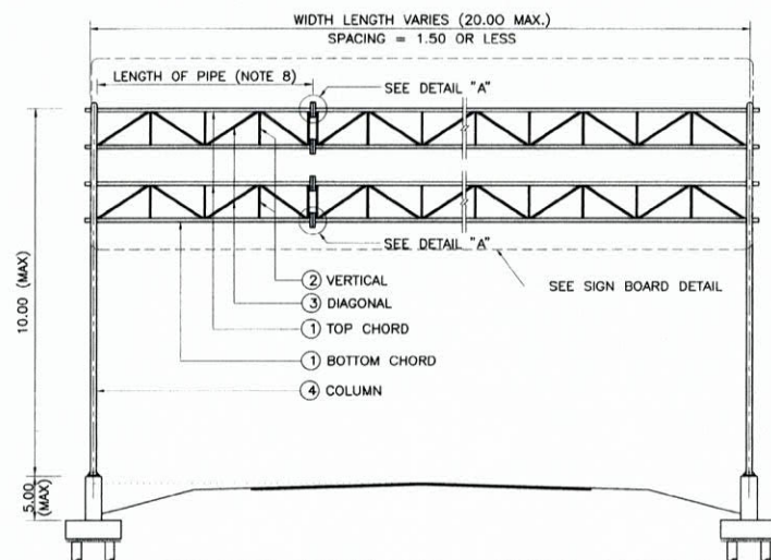
FOR SIGN BOARD 3.01 < \text{HEIGHT} \leq 5.20 M.
