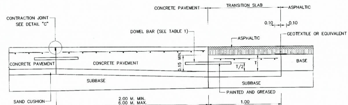
DETAIL OF JOINT BETWEEN CONCRETE PAVEMENT AND FLEXIBLE PAVEMENT
