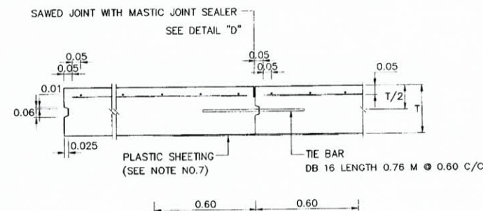
DETAIL OF LONGITUDINAL JOINT
