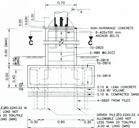
SECTION A - A SCALE 1:20
