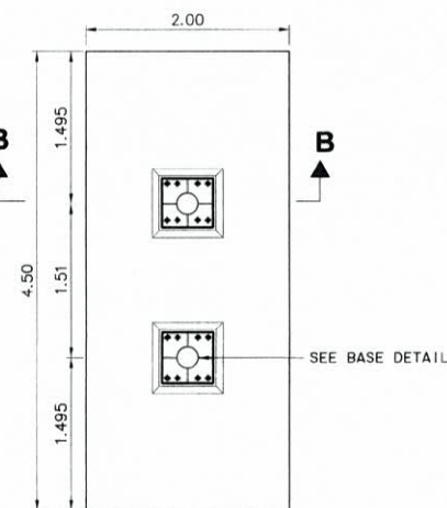
SPREAD FOOTING PLAN SCALE 1:40
