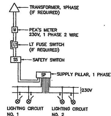
BLOCK DIAGRAM 3
