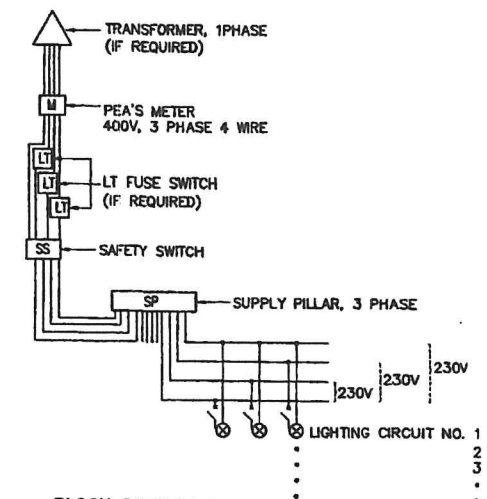
BLOCK DIAGRAM 4
